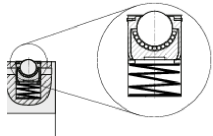
KLF - springloaded ball bar
